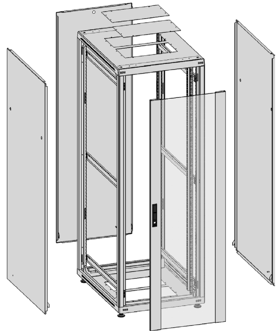
IMAGE® PRIMARY CABINET 600 mm deep
