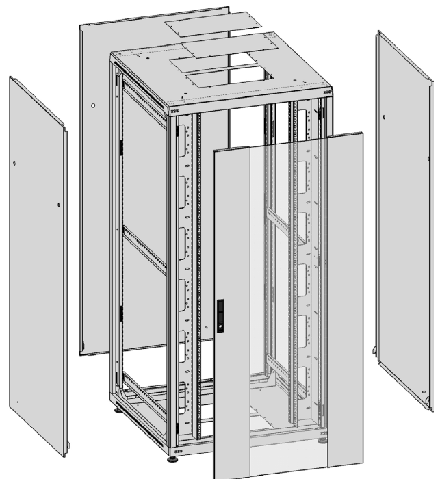
IMAGE® PRIMARY CABINET 800 mm deep
