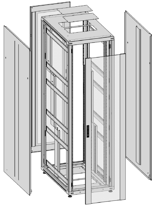
IMAGE® SERVER PRIMARY CABINET 1000 mm deep
